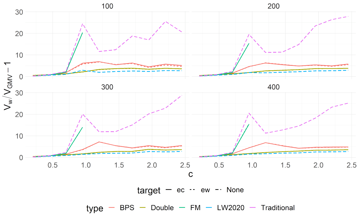
Figure 2: Relative loss V_w/V_{GMV} - 1 computed for several estimator of the GMV portfolio weights under scenario 1. Notice that some methods use different targets but are of the same type.
